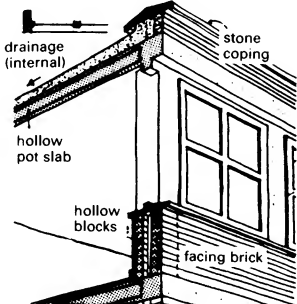
⑥ Reinforced concrete building with supports in external wall, fronted by outer leaf of parapet wall supported by the cantilevered floor
